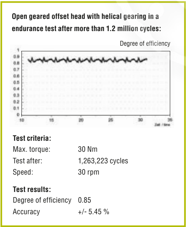
Right: Results of an endurance test.
